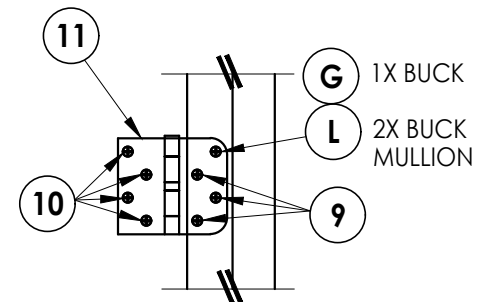
HINGE DETAIL 2
