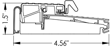
25 OUTSWING THRESHOLD
