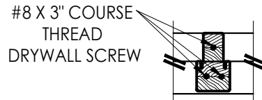
DETAIL 2
