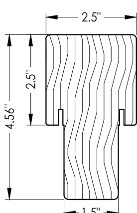
2 INTEGRAL MULLION
