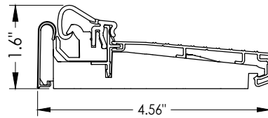
22 INSWING ARTICULATING THRESHOLD ZAC4565RDS
