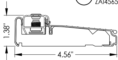
16 INSWING ADJUSTABLE THRESHOLD
