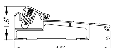
20 INSWING ARTICULATING THRESHOLD ZACLA4565
