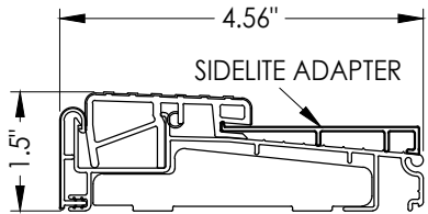
61 OUTSWING THRESHOLD w/ SIDELITE ADAPTER
