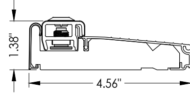
14 INSWING ADJUSTABLE THRESHOLD ZAI4565FN
