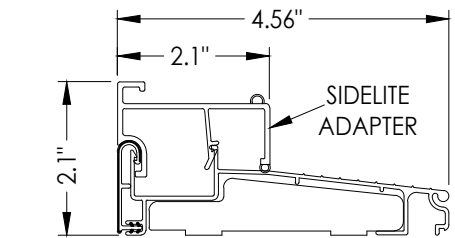
60 INSWING THRESHOLD w/ SIDELITE ADAPTER
