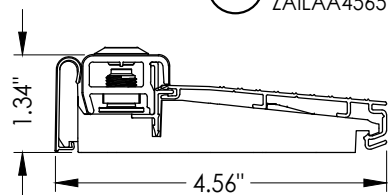
17 INSWING ADJUSTABLE THRESHOLD
