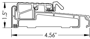
23 OUTSWING THRESHOLD
