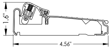
21 INSWING ARTICULATING THRESHOLD
