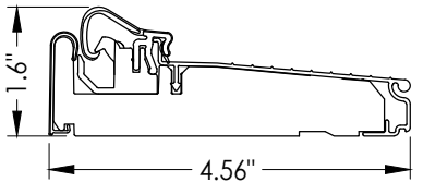
19 INSWING ARTICULATING THRESHOLD
